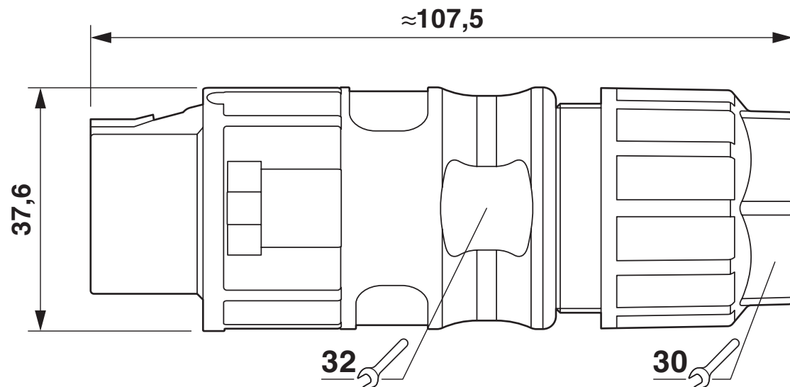
Dimensional drawing
