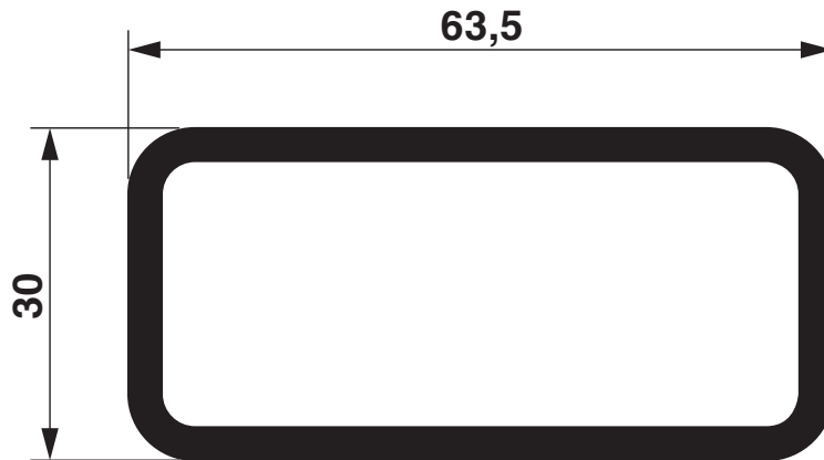
Dimensional drawing
