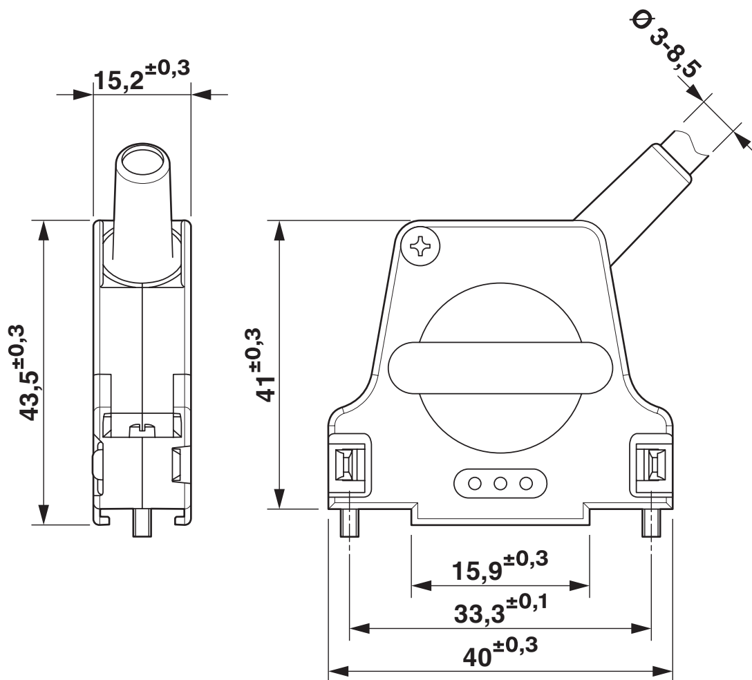
D-SUB sleeve housings
