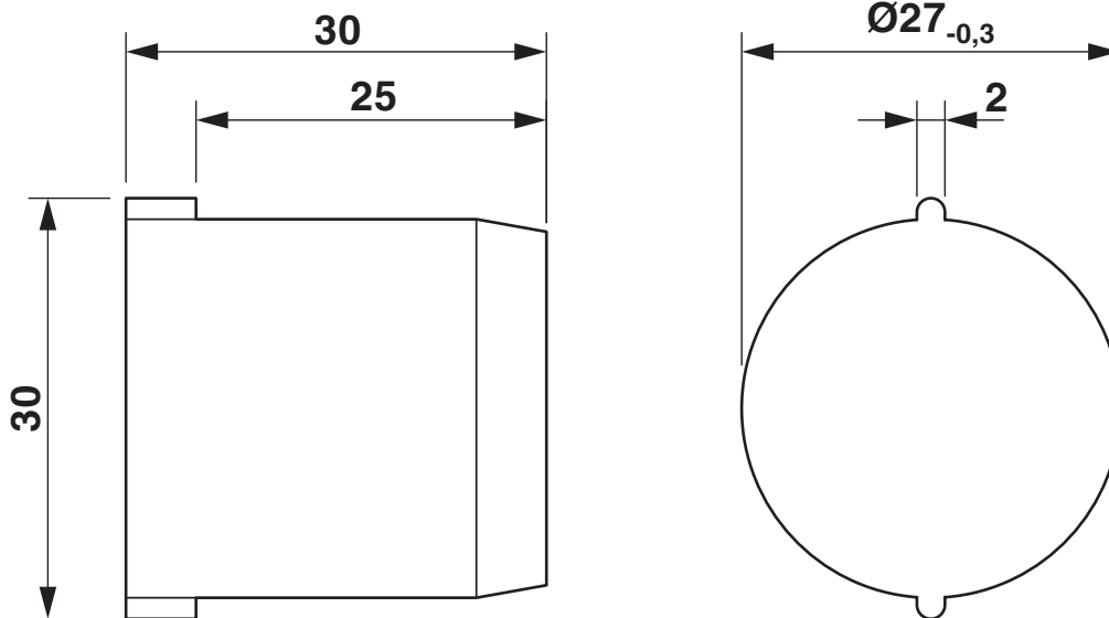
Dimensional drawing
