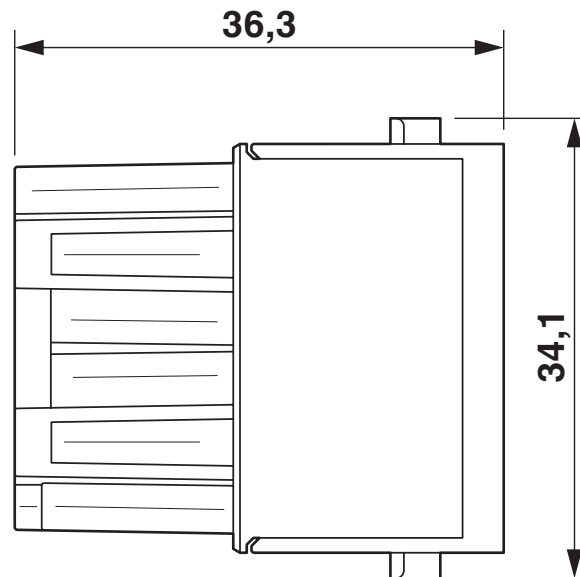
Dimensional drawing
