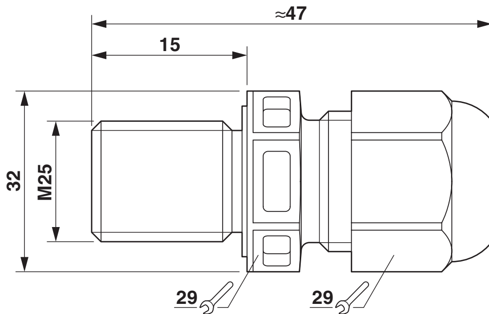
Dimensional drawing
