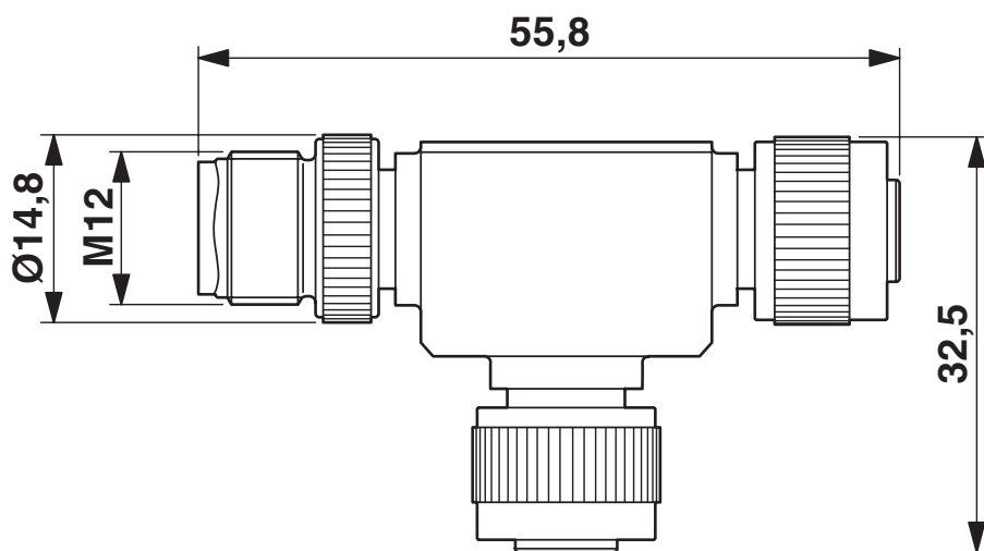
Dimensional drawing
