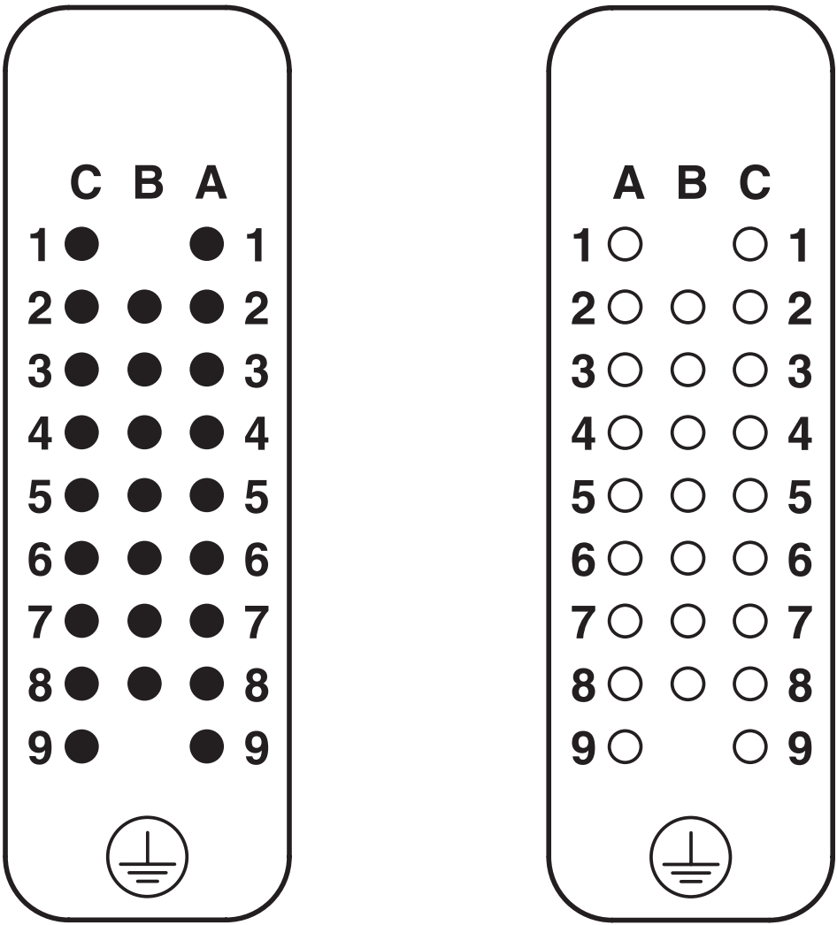
Schematic diagram
