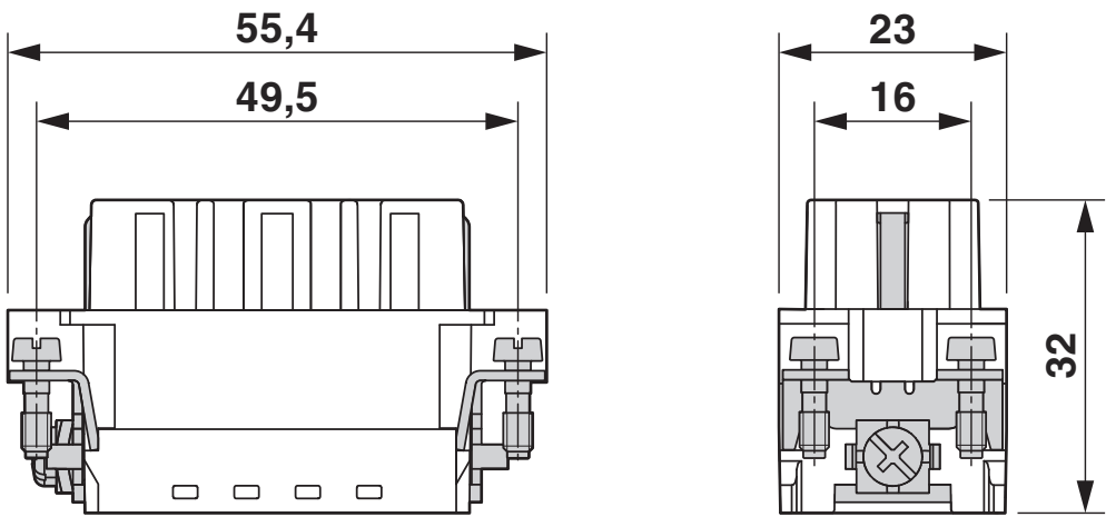
Dimensional drawing
