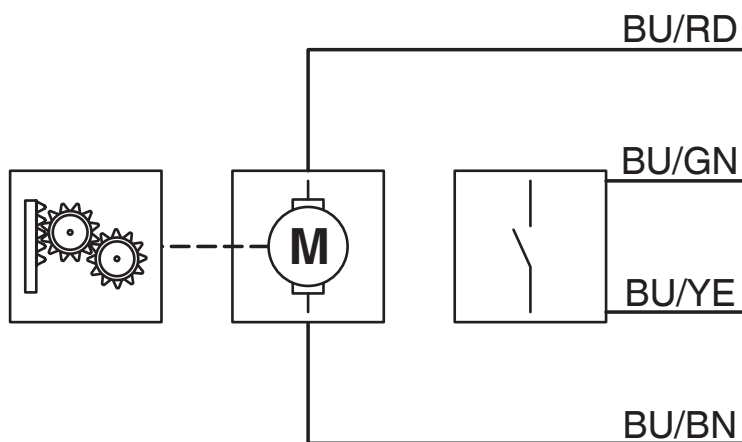
Block diagram
