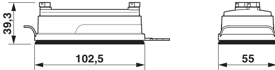
Dimensional drawing
