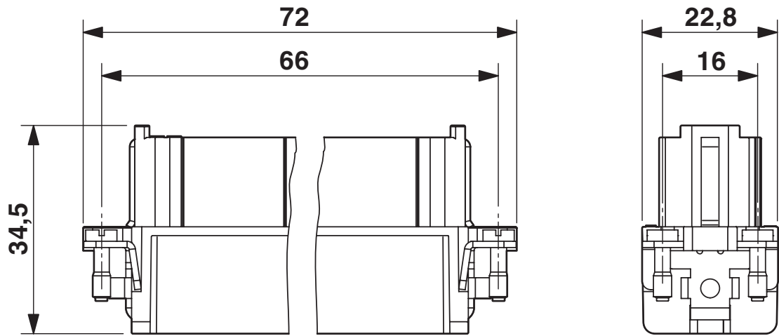
Dimensional drawing
