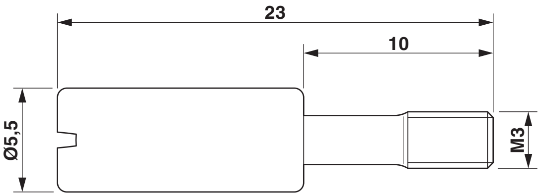
Dimensional drawing
