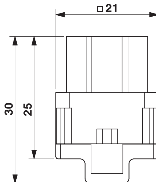
Dimensional drawing
