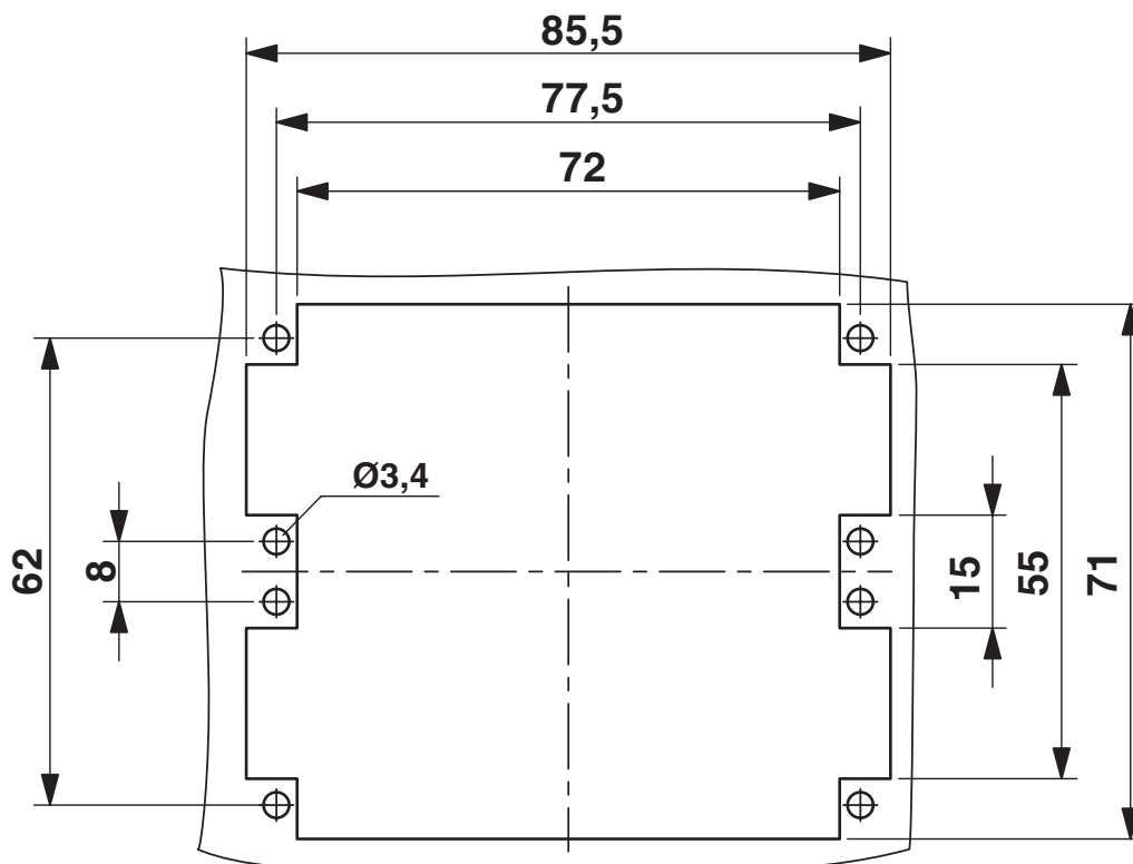
Dimensional drawing
