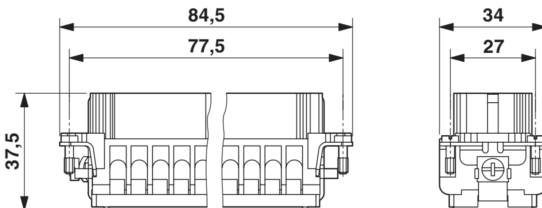
Dimensional drawing
