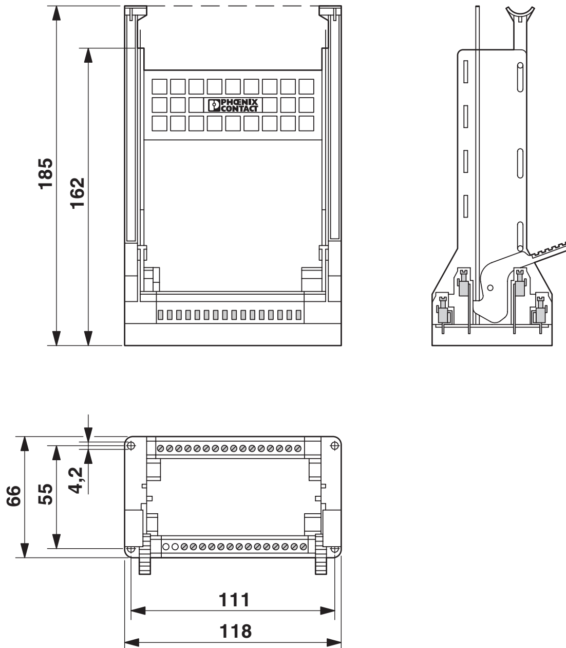
Dimensional drawing
