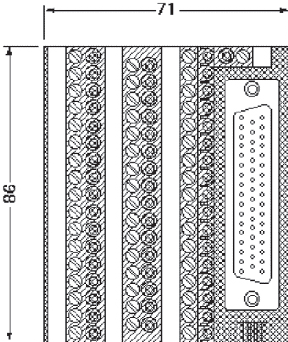
Dimensional drawing
