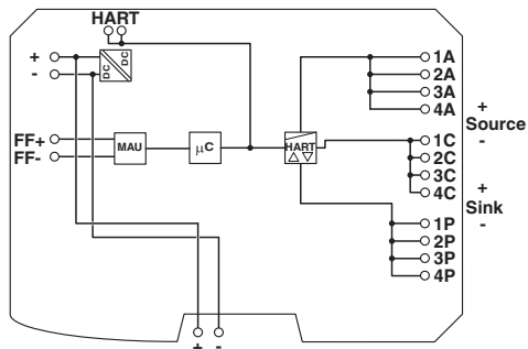
Block diagram
