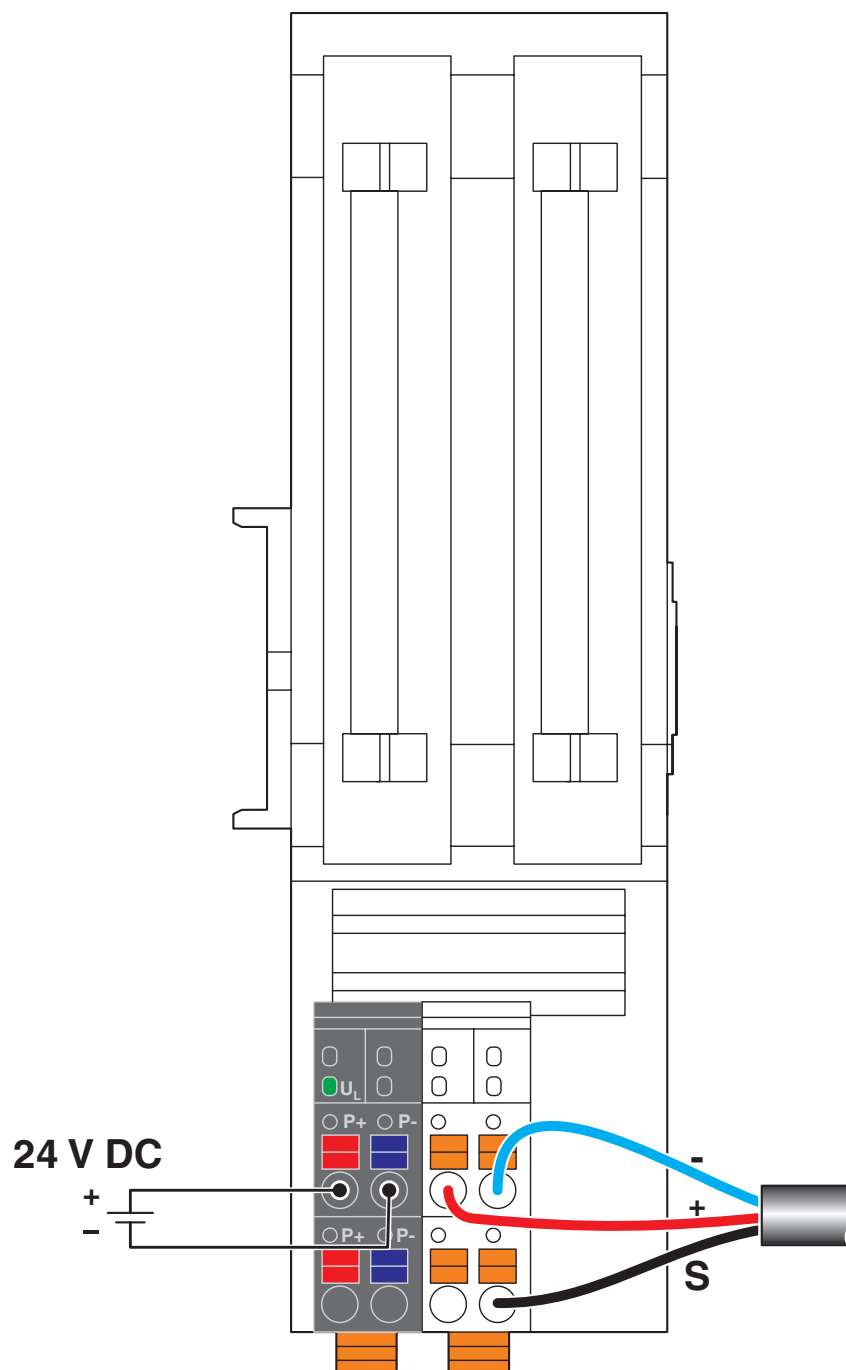
Connection diagram
