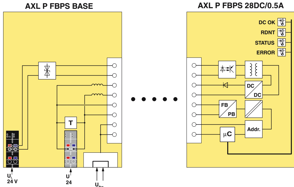
Block diagram
