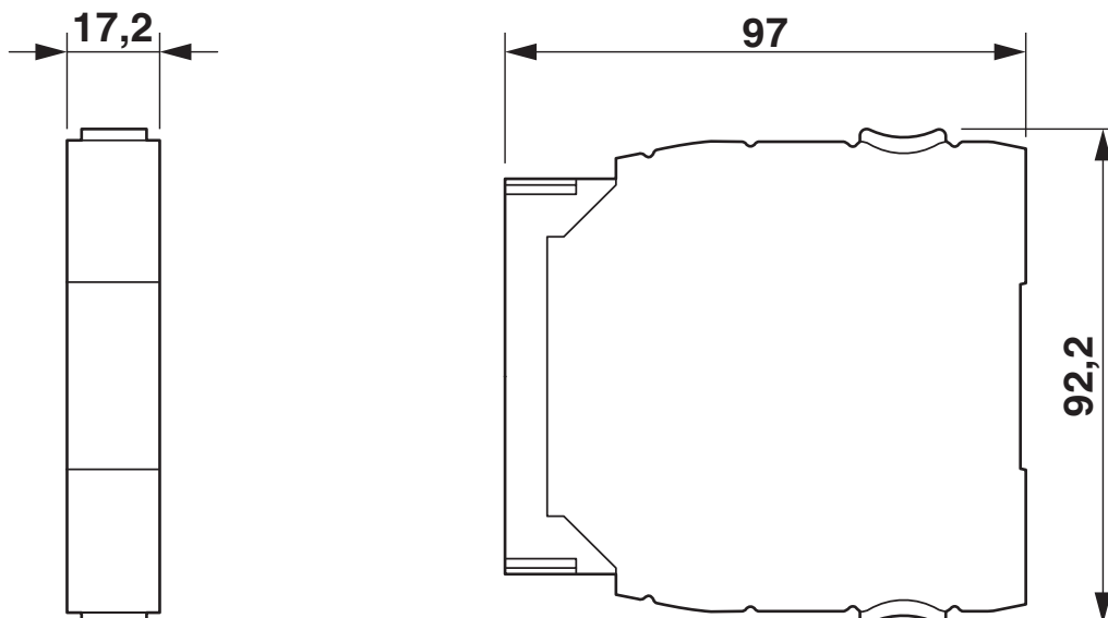
Dimensional drawing
