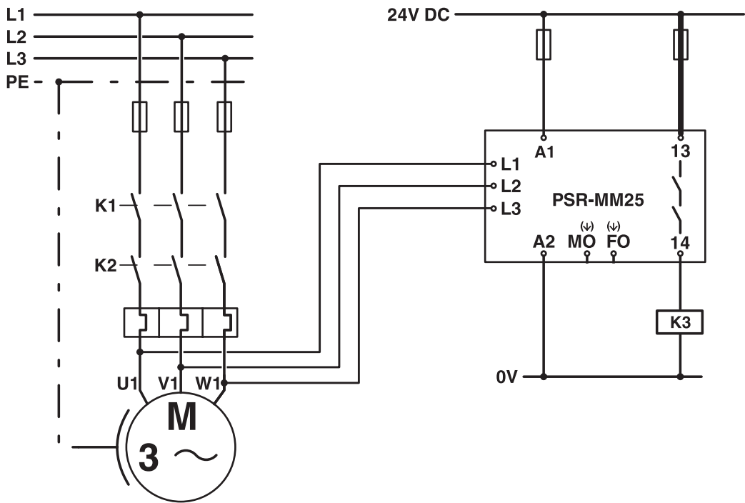
Circuit diagram
