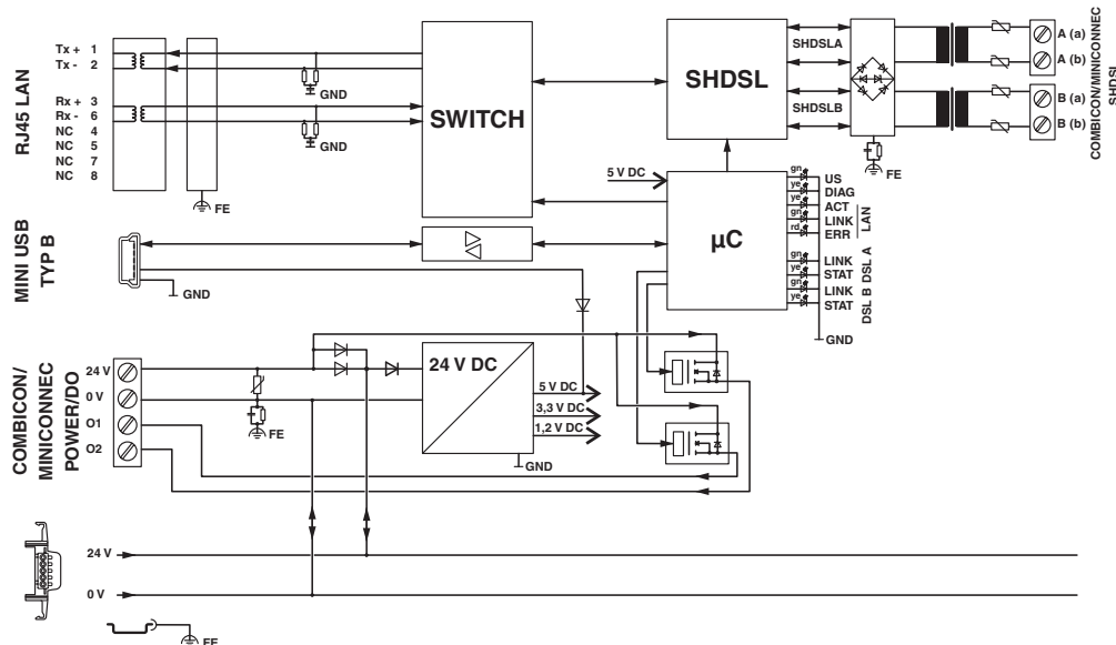
Circuit diagram
