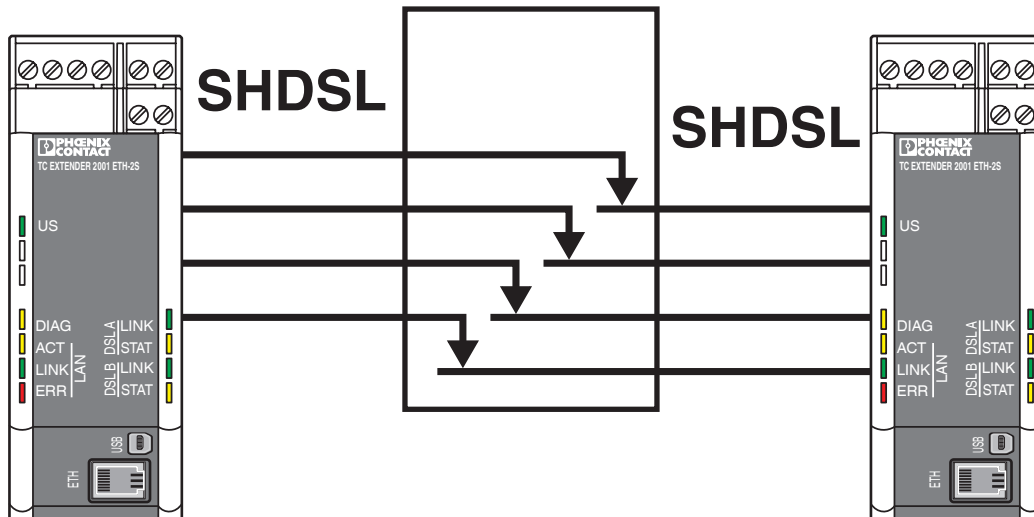
Application drawing
