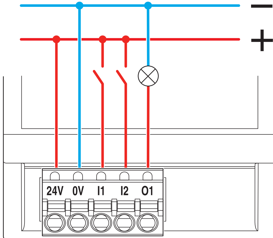
Connection diagram
