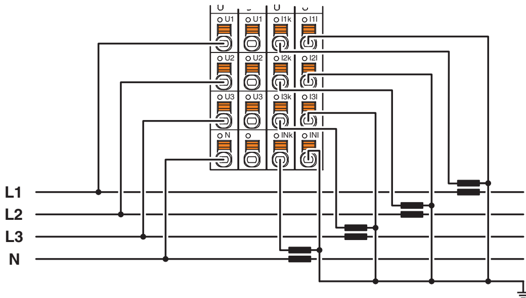
Connection diagram
