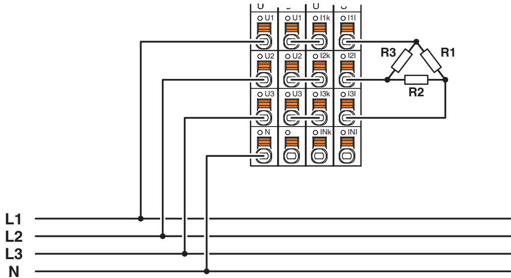
Connection diagram
