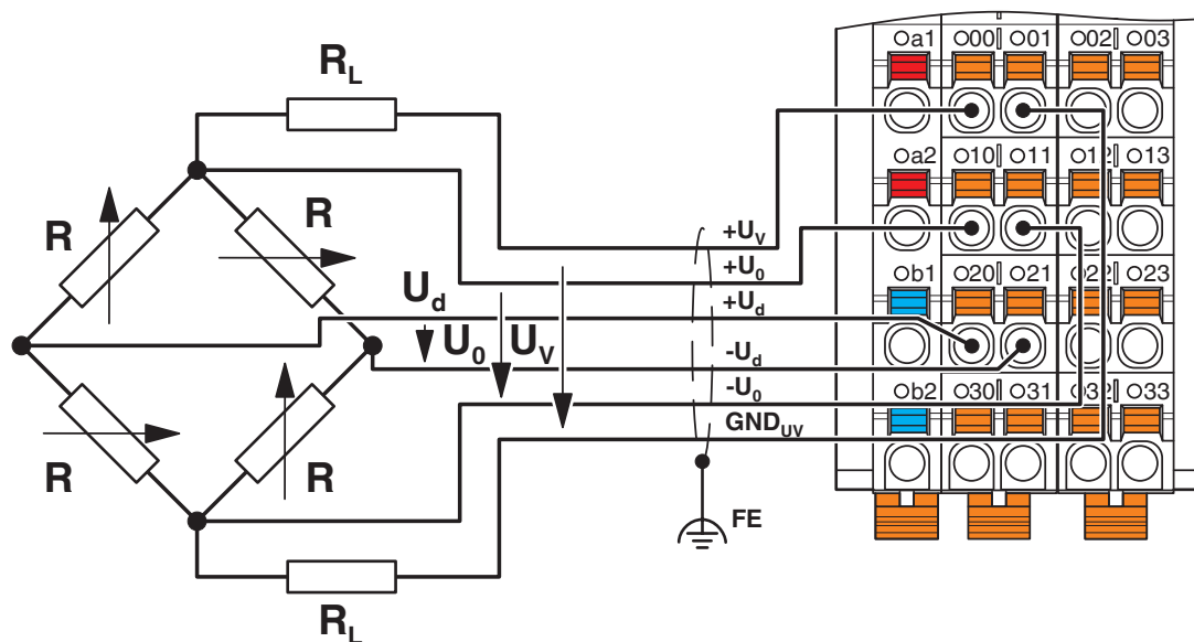
Connection diagram
