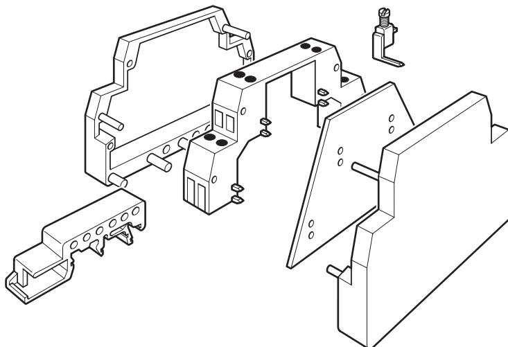
Exploded view
