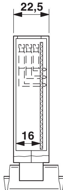
Dimensional drawing
