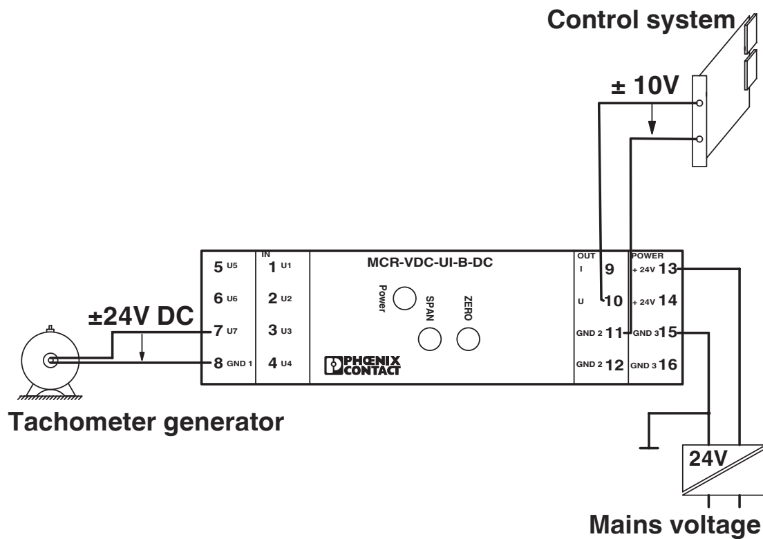
Application drawing
