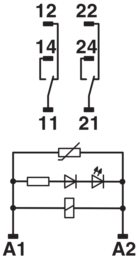
Circuit diagram
