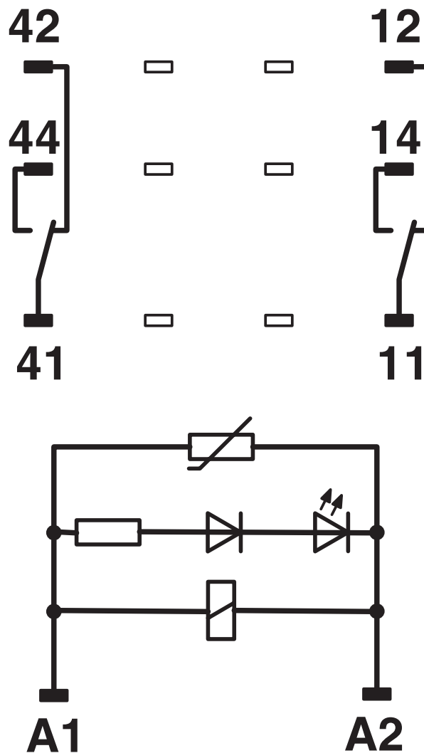
Circuit diagram
