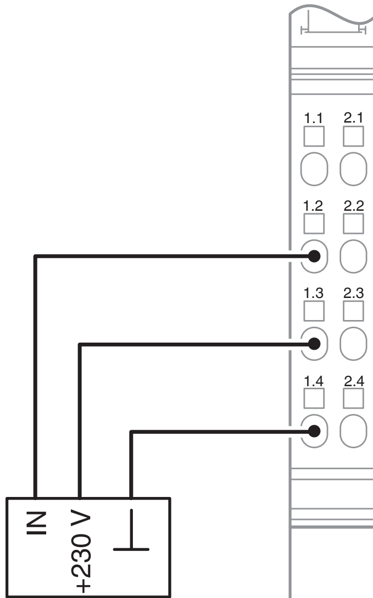
Connection diagram
