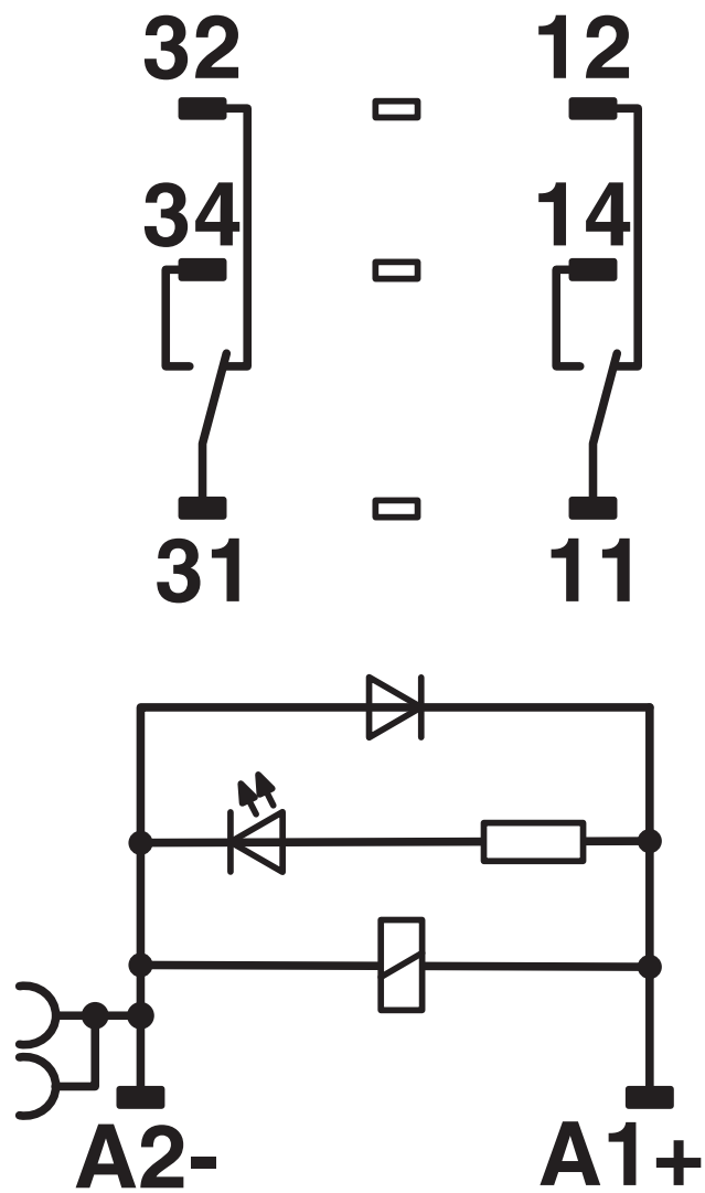
Circuit diagram
