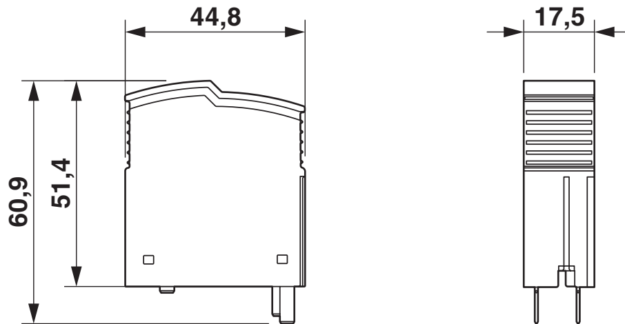
Dimensional drawing
