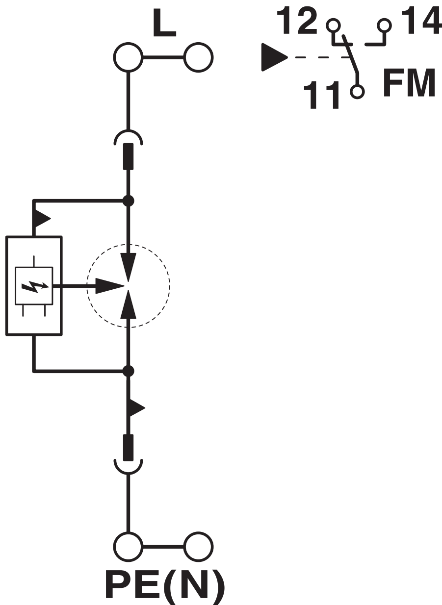
Circuit diagram
