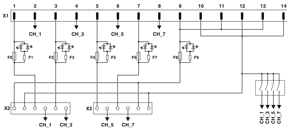
Circuit diagram
