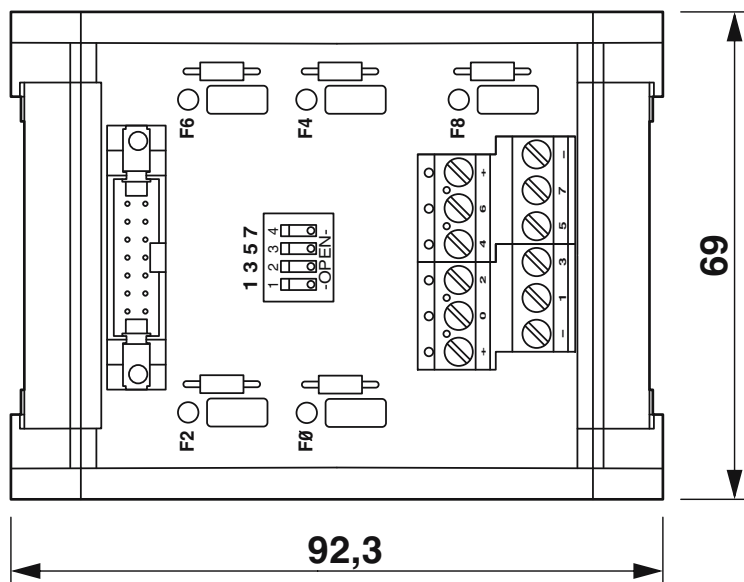
Dimensional drawing
