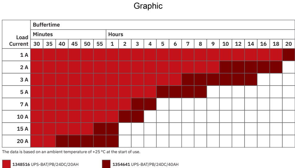
Buffer times for TRIO DC UPS for lead battery module
