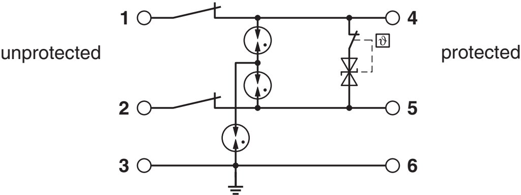
Circuit diagram
