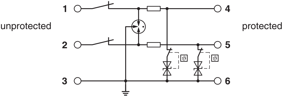
Circuit diagram
