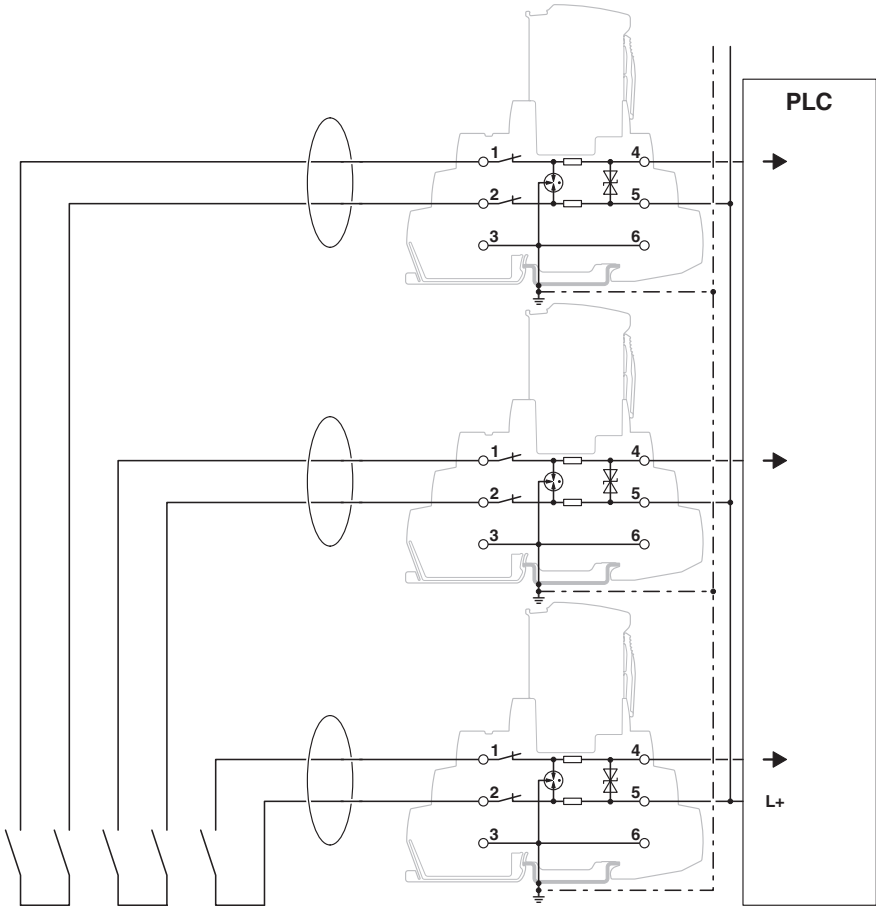
Application drawing
