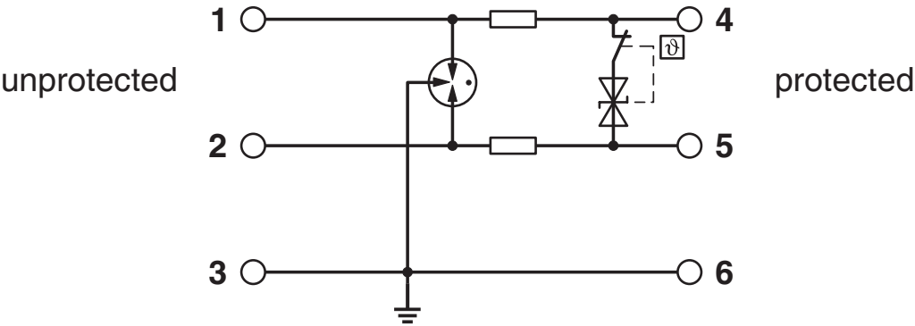
Circuit diagram
