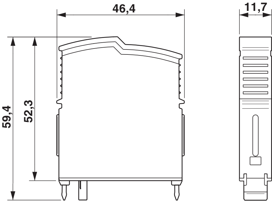
Dimensional drawing
