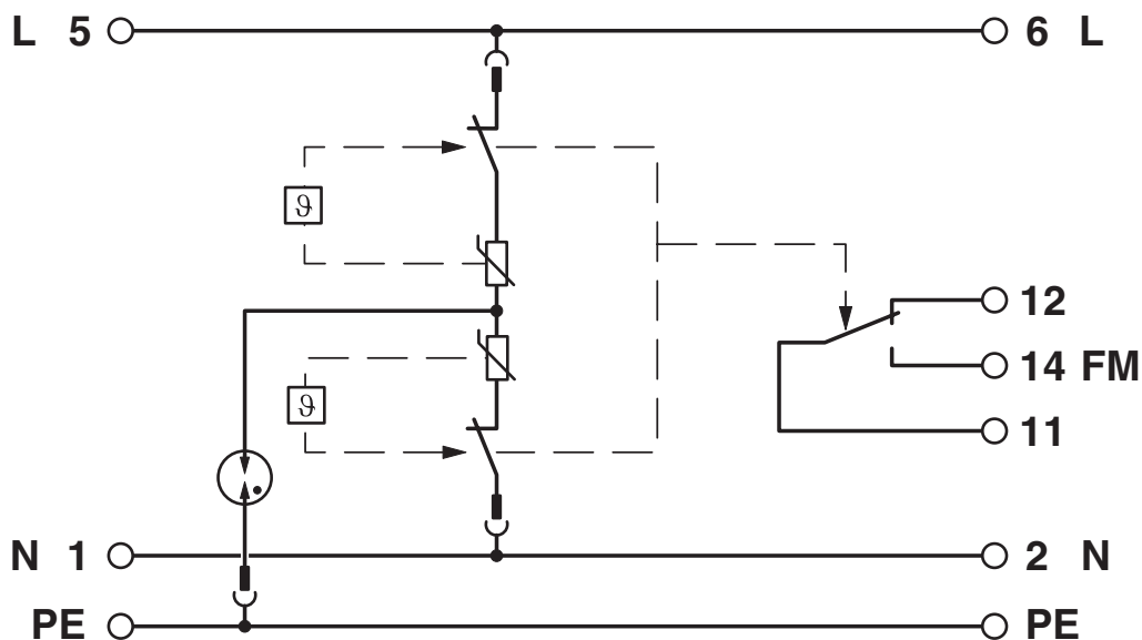
Circuit diagram
