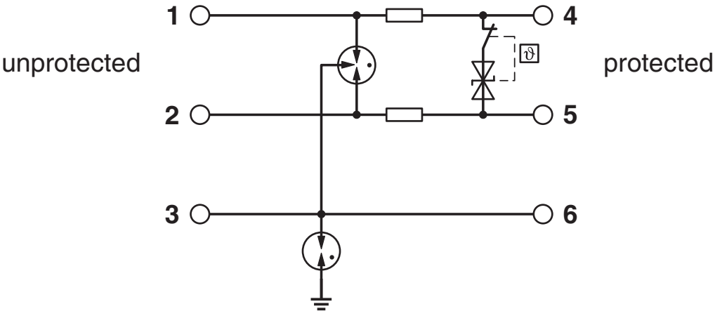
Circuit diagram
