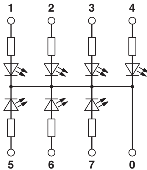
Circuit diagram
