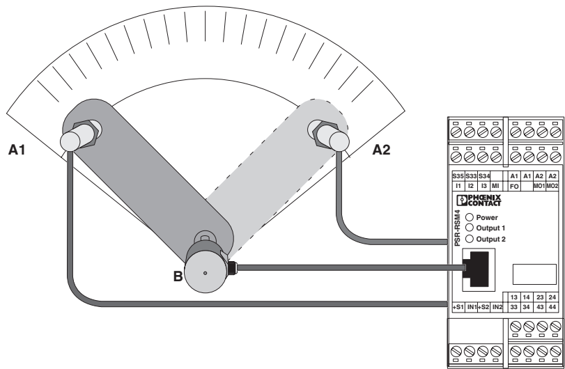
Application drawing
