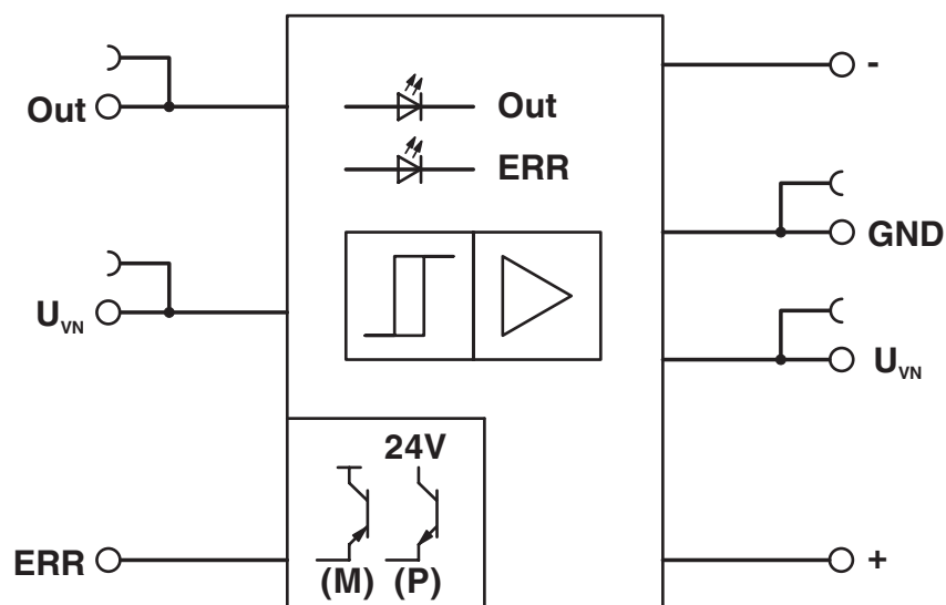
Circuit diagram
