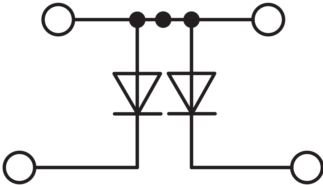
Circuit diagram
