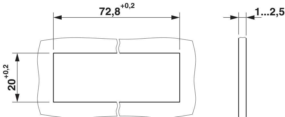
Dimensional drawing
