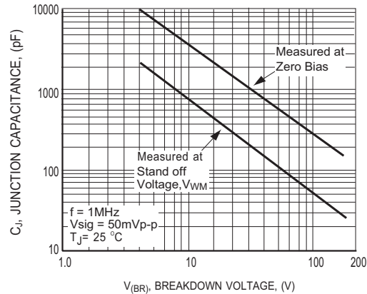
FIG.4 TYPICAL JUNCTION CAPACITANCE BIDIRECTIONAL
