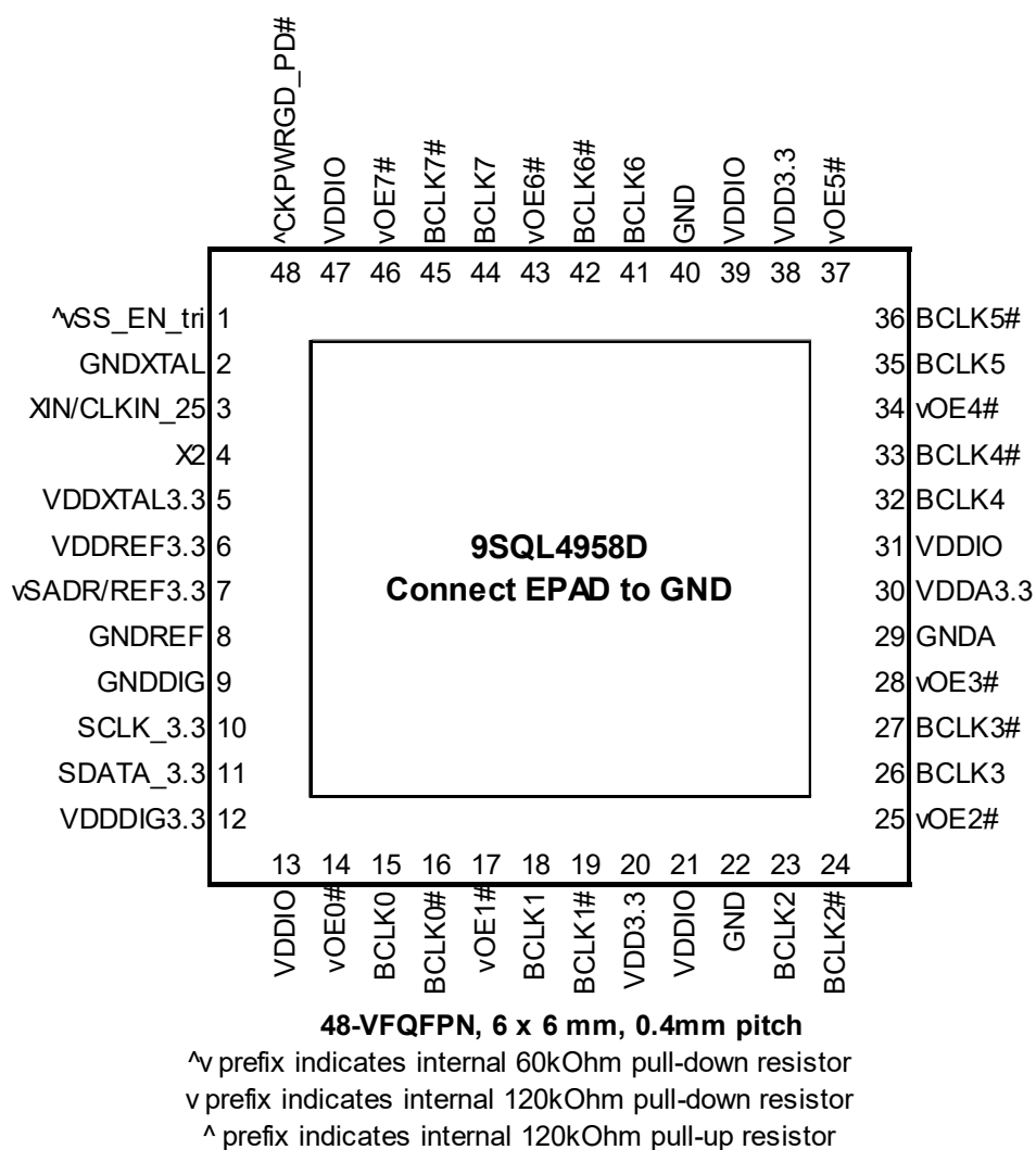
Figure 4. Pin Assignments for 6 × 6 mm 48-VFQFPN Package – Top View
